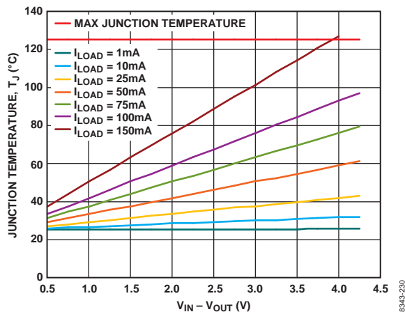
Figure 35. TSOT, 0 mm 2 of PCB Copper, T A = 25°C
